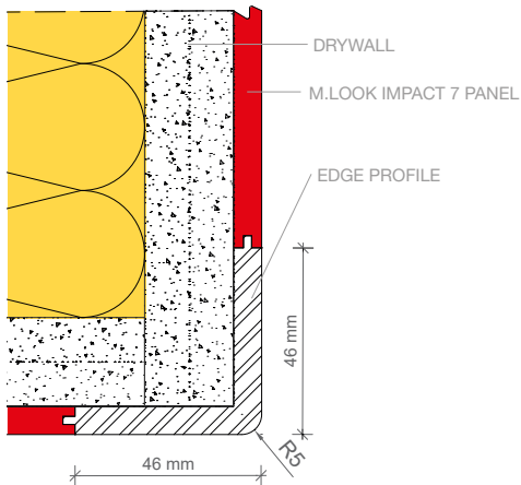
OUTSIDE CORNER DETAIL A104
