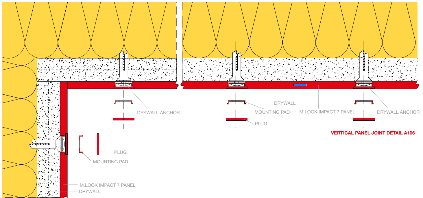
INSIDE CORNER A105
