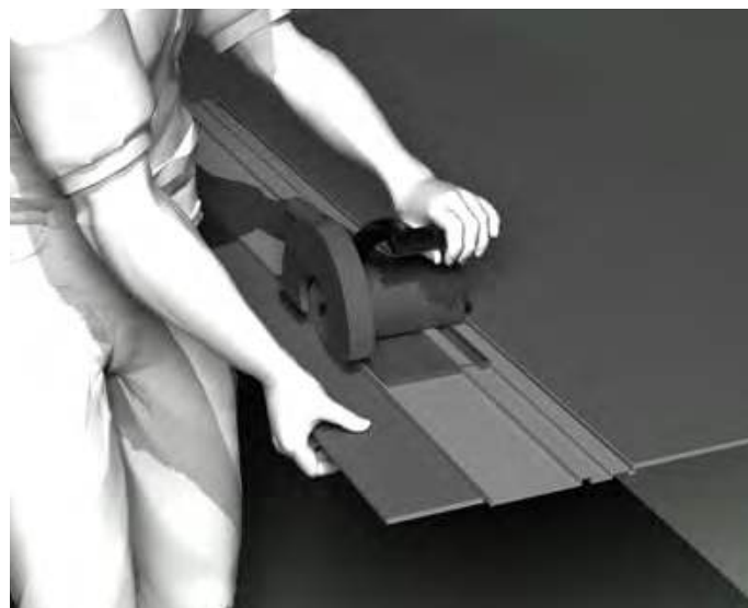
Final cut
